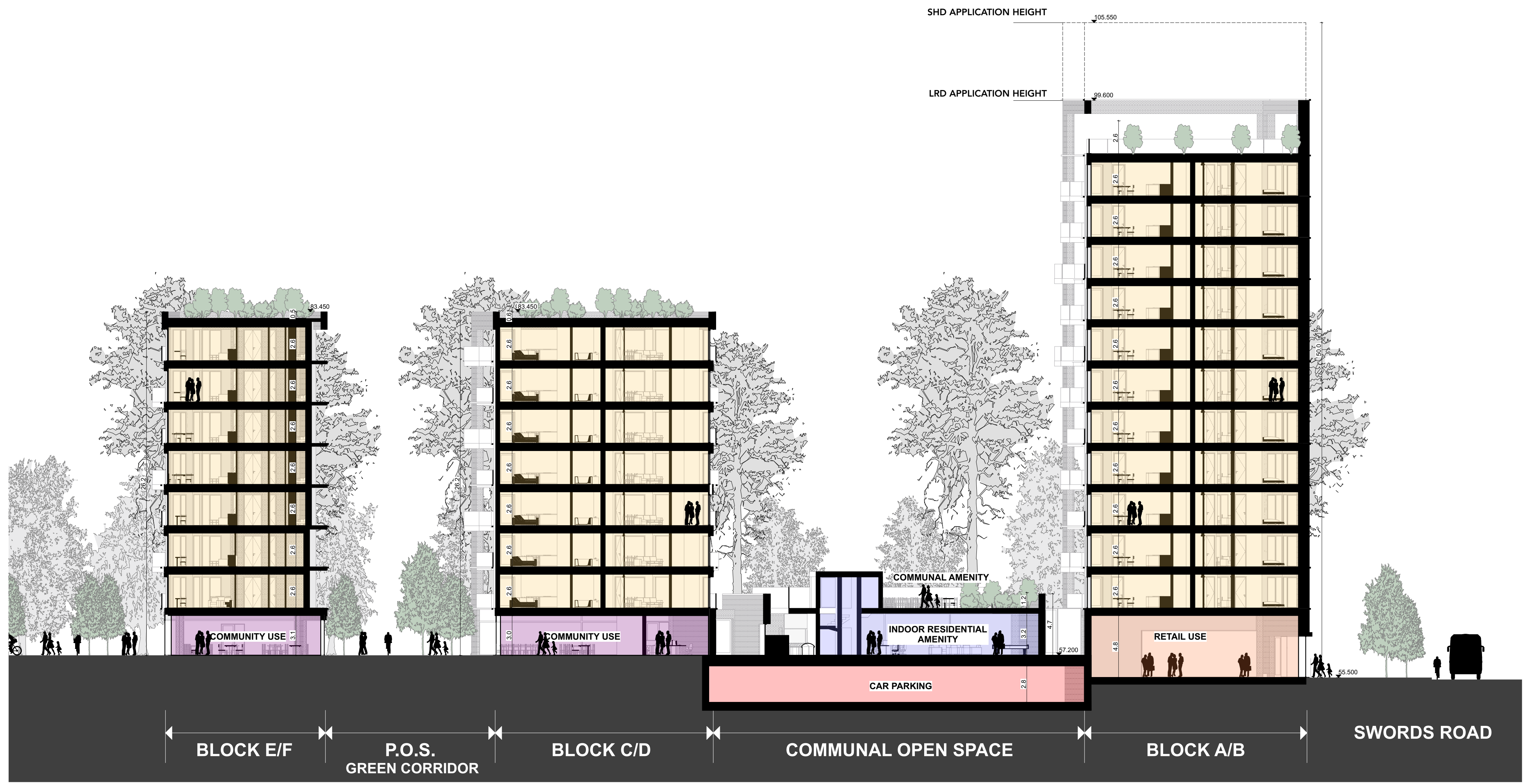
Section L-L SCALE : 1:200
